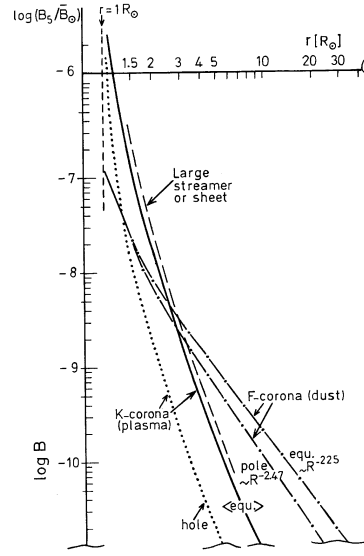
Figure 1. Radial variations of intensities for various components of the solar corona (Koutchmy & Lamy, 1985). Notice the logarithmic scales.
