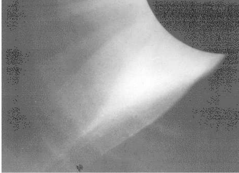
Figure 6. Portion of a picture of the 1961 corona (observation: M. Laffineur – IAP/CNRS) obtained on plate, with compensation of the radial gradient using a mechanical system. Around the streamer in bulb, a quasi-cylindrical sheet with tangential discontinuity is identifiable (see arrow). This historical picture was reproduced many times, e.g., Menzel (1961), Billings (1966).
