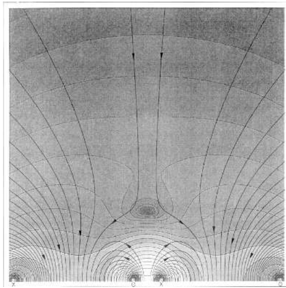
Figure 3. Axisymmetric numerical model of a simple structure of magnetic field induced by a horizontal loop of current located near the surface, and surrounded by another loop much wider and coaxial. Notice the null point or singularity of the field, into dark, at the top of the loops. The lines of field are drawn, some with arrows, indicating the direction, and the local value of the magnetic pressure is coded in hues of gray.
