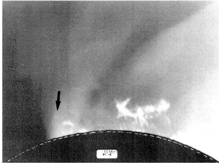
Figure 5. Portion of field in the vicinity of the E-limb of the 1991 corona, with the plasmoide (see the arrow) at the beginning of the sequence. Image taken with a red filter and a photographic film with a filter neutral radial and an exposure time of 20 s. The position of the limb of the Sun behind the Moon is indicated.
