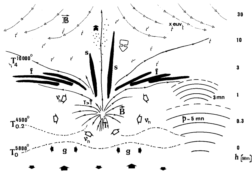
Figure 2. Very schematized representation of the solar surface in the vicinity of an element of the chromospheric network with concentration of magnetic field in the photosphere. The thick arrows indicate the field of velocities. Notice the logarithmic scale of heights H ; B -magnetic field; T -temperatures; V_h -horizontal speeds; G -granulation; S -spicules; F -fibrils.
