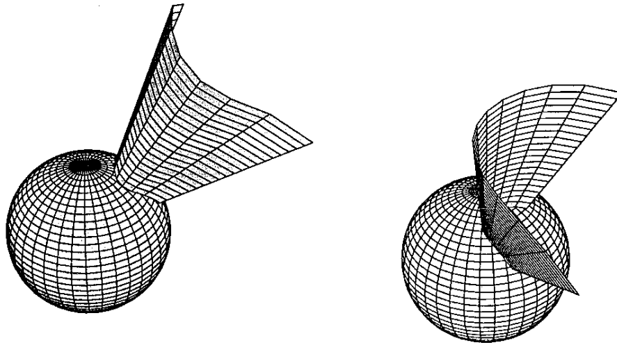
Figure 8. Simulation intended to illustrate the effects of projection met during the interpretation of the images of an eclipse corona. Notice that a curved layer can easily show a discontinuity.
