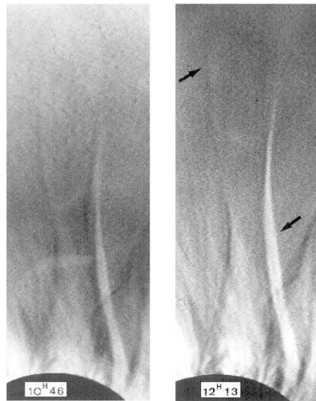
Figure 7. Portion of the June 30, 1973 eclipse corona obtained on film-sheet using a radial neutral filter. On left, by a team of the Observatory of Kiev operating in Mauritania; on the right by the team of the IAP (CNRS) operating in Chad. On the edge of this large streamer which shows a discontinuity, a phenomenon of detachment (see the arrow) or disconnection have been observed for the first time, undoubtedly showing an instability of a new type, which itself propagates radially with a speed which have been measured using these observations and which have been found equal to 140 km/s.
