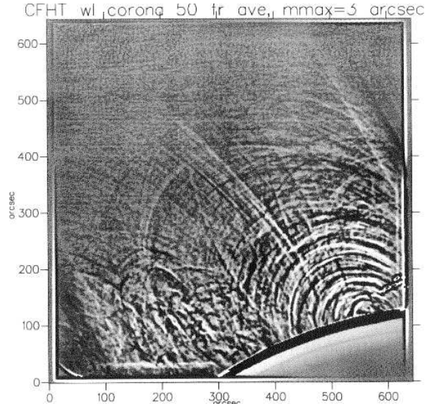
Figure 4. Undoubtedly the image of the corona obtained with the best resolution ever reached on such a field of view. Observation carried out with the CFHT at the eclipse of 1991, at the primary focus, with a camera of 70 mm format, on film 6415 exposed 1/60 s with a rate of 2 images/s. Digital processing using an algorithm intended to show the dominant gradients at 3'' scales.
