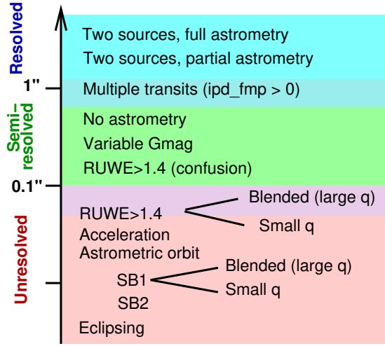
Figure 2. Schematic inventory of binarity indicators in Gaia. They are split into three broad groups: resolved (wide), semi-resolved, and unresolved (close) binaries. Each indicator has a complex and poorly known selection bias.
