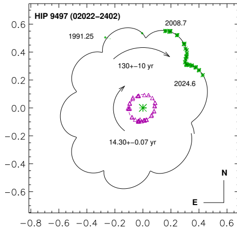
Figure 1. The double twin triple system HIP 9497 with recently updated orbits (Tokovinin, 2018a). The inner 14.3-yr orbit is well constrained, and the still uncertain outer period suggest a period ratio of 1:9, possibly in a mean motion resonance. Both orbits are quasi-circular. The masses of two stars in the inner pair are 0.6 M_{\odot} , the primary is of 1.2 M_{\odot} .
