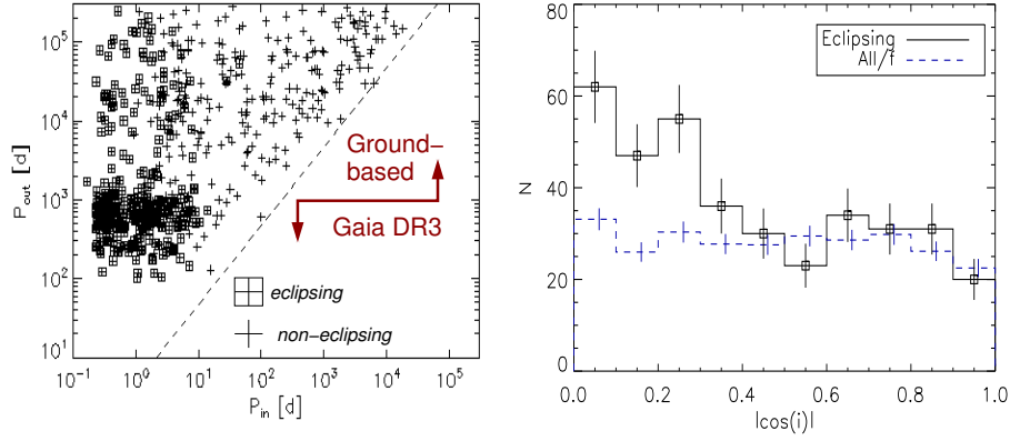
Figure 3. Mutual alignment in triple systems containing EBs. The left panel is a plot of outer and inner periods of all hierarchies with known outer inclinations. Outer periods below 1000 days are dominated by the Gaia sample of Czavalinga et al. (2023), longer periods result from ground-based observations. The dashed line is the dynamical stability limit; eclipsing subsystems are marked by squares. The right panel plots the histogram of x = |\cos i| in the 369 hierarchies containing EBs and the scaled-down histogram for all hierarchies with known inclinations.
